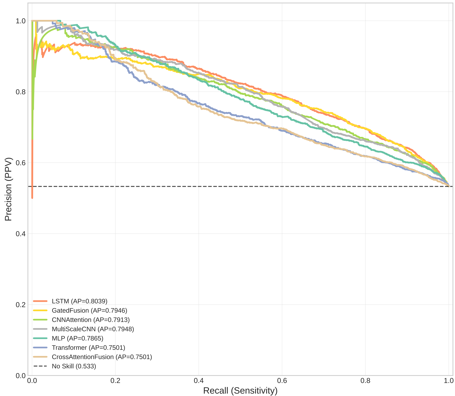
Precision-Recall Curves
